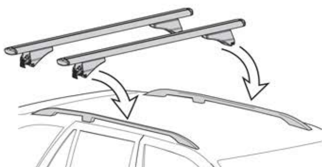
Raised rails
